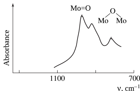
Fig. 1. IR spectrum of the Sn–Mo oxide catalyst in the region of inherent vibrations recorded in KBr pellets with compensation by the SnO 2 sample.
