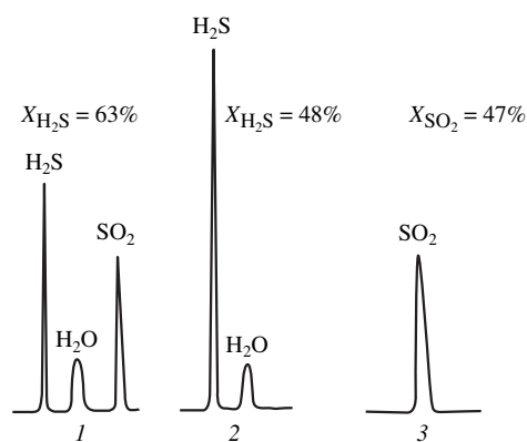
Fig. 2. Chromatograms and calculated conversions of \text{SO}_2 and \text{H}_2\text{S} on the stationary surface of the Sn–Mo oxide catalyst at combined (1) and separate (2, \text{H}_2\text{S} ; 3, \text{SO}_2 ) pulse feed of reactants. [\text{H}_2\text{S}] = 0.175 vol %, [\text{SO}_2] = 0.09 vol %; T = 523 K. The portion of \text{H}_2\text{S} converted in the pulse is 14% of the monolayer.
