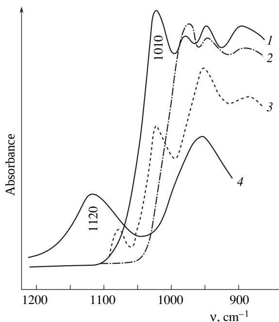
Fig. 4. IR spectra of (1) initial Sn–Mo oxide catalyst oxidized at 723 K; (2) after treatment with water at 293 K; (3) after reduction with \text{H}_2 at 523 K followed by evacuation at 673 K; and (4) after treatment with \text{H}_2\text{S} (10 Torr) at 298 K for 30 min.
