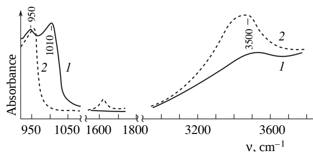
Fig. 3. IR spectra of the Sn-Mo oxide catalyst (1) oxidized at 723 K and (2) after interaction with water at 293 K.
