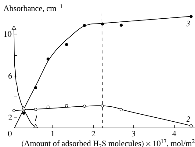
Fig. 7. Changes in the absorbance of the absorption bands of adsorbed \text{SO}_2 during interaction with \text{H}_2\text{S} at 293 K: (1) 1330, (2) 1080, and (3) 1620 \text{cm}^{-1} .
