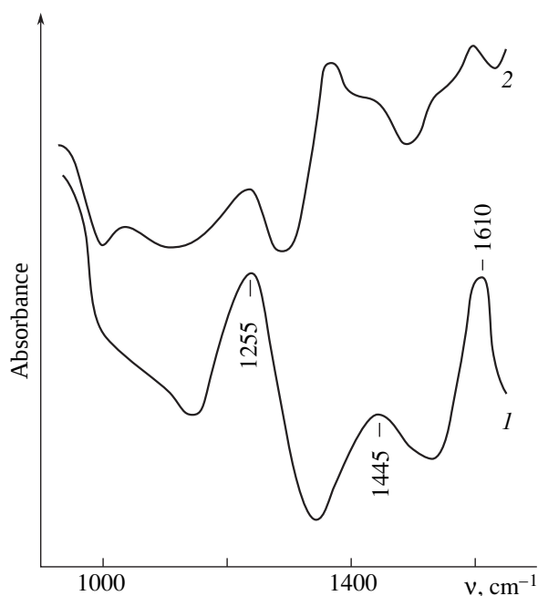
Fig. 5. IR spectra of ammonia adsorbed on the oxidized surface of the Sn-Mo oxide catalyst (1) before and (2) after interaction with \text{H}_2\text{S} .
