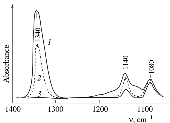
Fig. 6. IR spectra of SO_2 adsorbed on the oxidized surface of the Sn\text{--}Mo oxide catalyst after adsorption of SO_2 (1) and (2) 10 Torr followed by desorption (3). T = 298\text{ K} .
